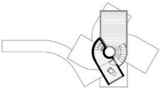
4th FLOOR PLAN
